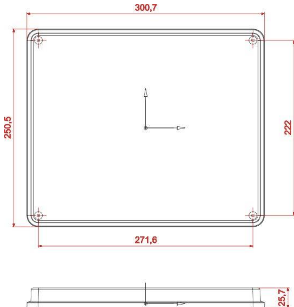
Product Drawing
